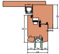
Vertical Section
