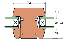
Vertical Muntin
