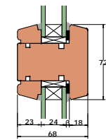
Horizontal Muntin
