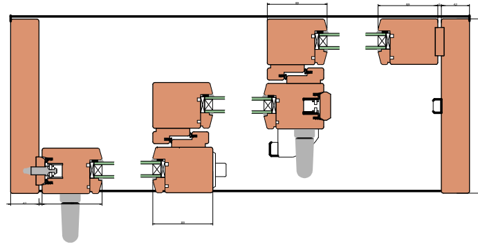
Scheme E Horizontal Section
