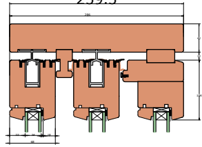
Vertical Section 259.5
