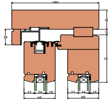
Vertical Section
