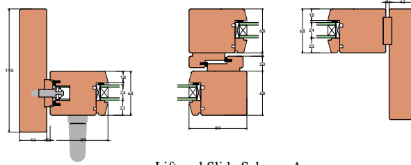
Lift and Slide Scheme A
