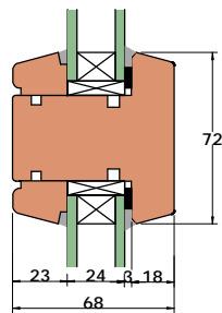
Horizontal Muntin
