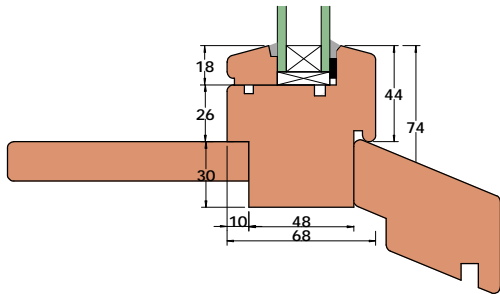
Horizontal Muntin
