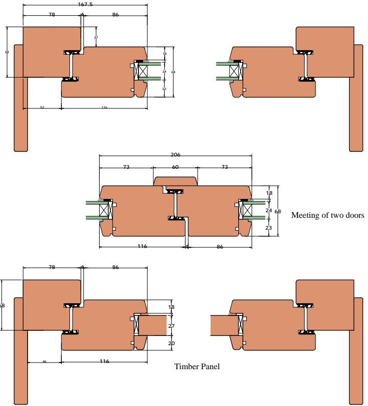
Horizontal Section
