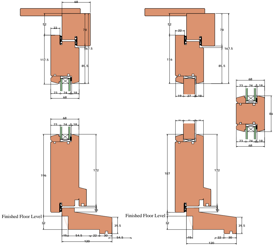
Vertical Section
