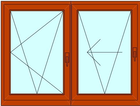
Tilt and Slide Scheme A with single open
