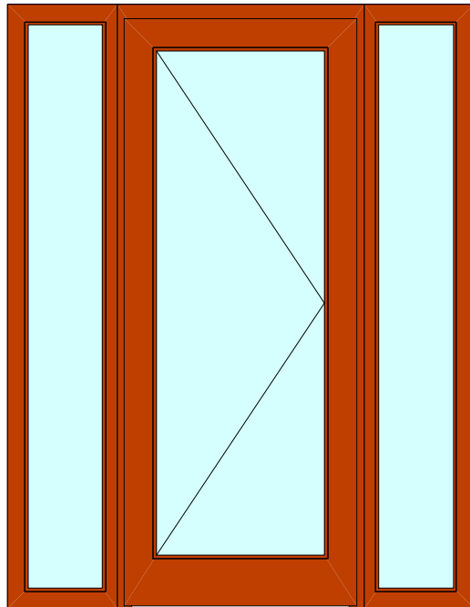
Glazed Entrance door w sidelites
