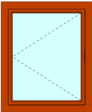
Single O/O window
