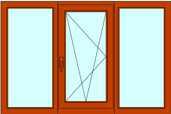
Single opening window w two fixed lites
